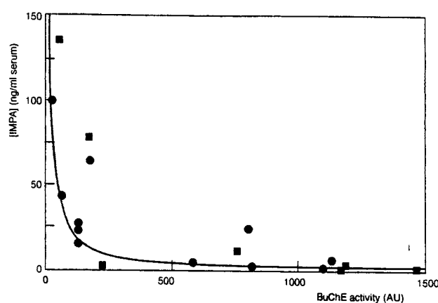
Fig. 3 Inhibition of butyrylcholinesterase (BuChE) activity in serum samples of victims of terrorist attacks with sarin in Tokyo (●) and Matsumoto (■), measured within 1.5 h after exposure, and concentration of hydrolysed sarin (IMPA) in these samples. The drawn curve follows the equation: [IMPA] = -0.70 + 25 \text{ BuChE activity} , with [IMPA] in ng/ml serum and BuChE activity in arbitrary units (AU)
