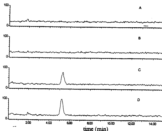
Fig. 2 Negative ion liquid chromatography (LC) tandem electrospray mass spectrometry (MS) using the multiple reaction monitoring scanning mode for transition m/z 137 \rightarrow m/z 95 (IMPA) or m/z 140 \rightarrow 98 (O-isopropyl trideuteromethylphosphonic acid; IMPA- d_3 ). Traces A and B (IMPA and IMPA- d_3 , respectively) represent a blank serum sample; traces C and D (IMPA and IMPA- d_3 , respectively) represent a Japanese serum sample (50 \mu l; second sample of victim no. 3) to which a solution of IMPA- d_3 (21 ng/ml; 50 \mu l) had been added. The LC system consisted of a microbore column (20 cm \times 320 \mu m) containing PRP-X100 (10 \mu m particles), with H_2O/CH_3CN (1:1, v/v), containing 0.5% HCOOH , as the eluent. Flow rate, 20 \mu l/min, injection volume, 2 \mu l
